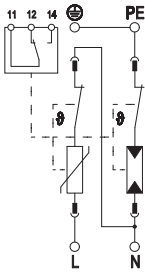
Connection options
