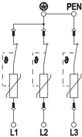
Connection options
