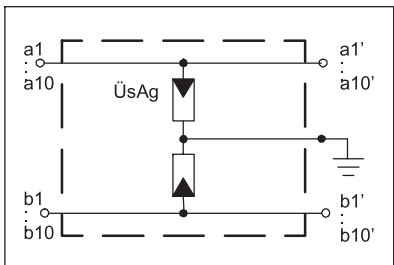
Connection options
