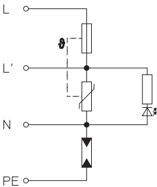
Connection options
