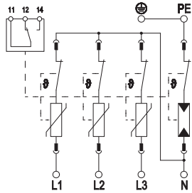
Connection options
