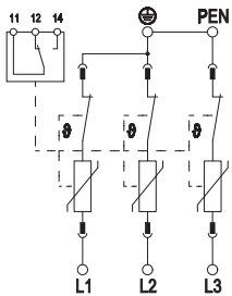
Connection options
