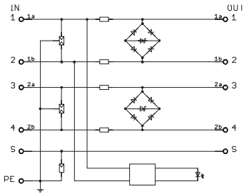
Connection options
