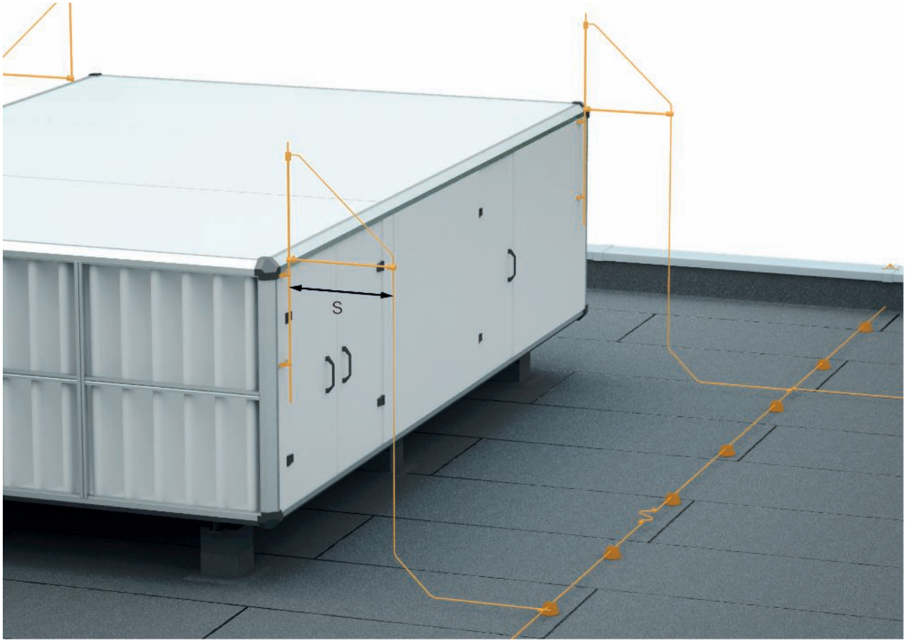
Correctly maintained separation distance (s) between down-conductor systems and roof structures
