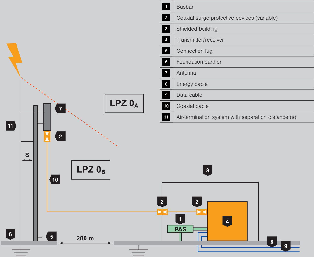
Insulated lightning protection on an antenna system and various earthing systems
