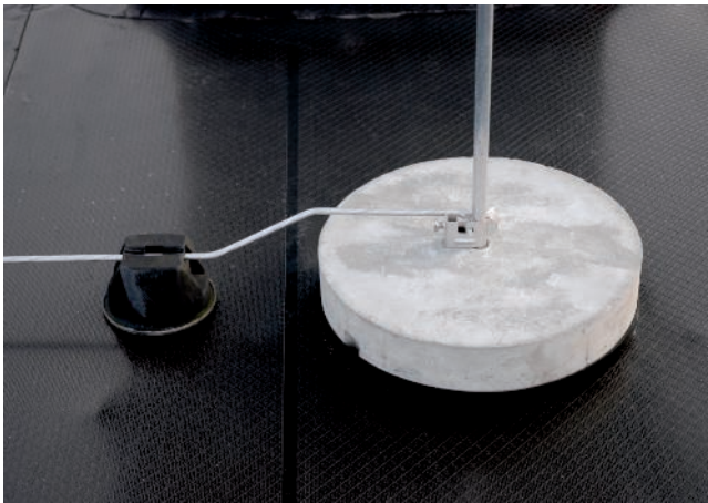
Air-termination rod
