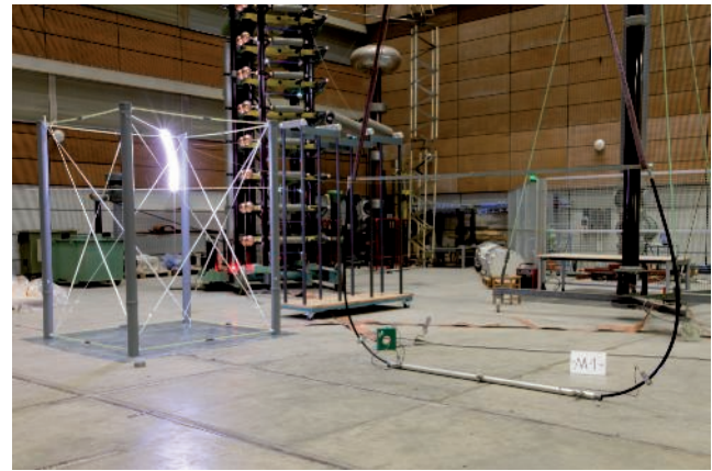
Testing structure during an impulse voltage test with an equivalent separation distance ( s_e ) of 75 cm.
