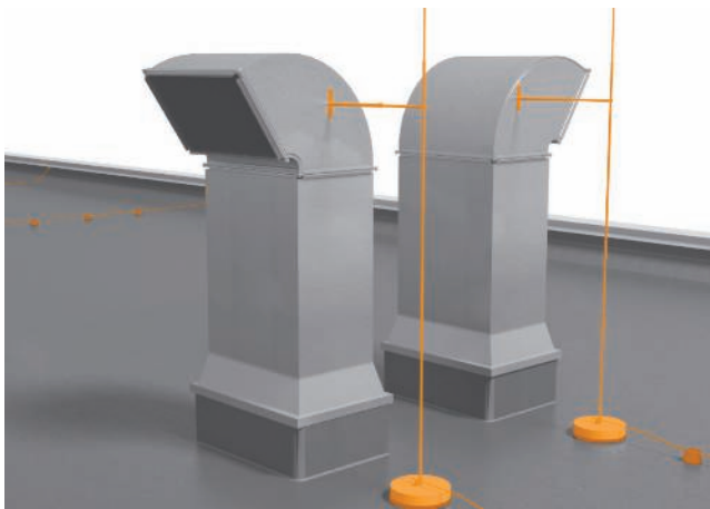
Air-termination rod with adjustable insulating beam
