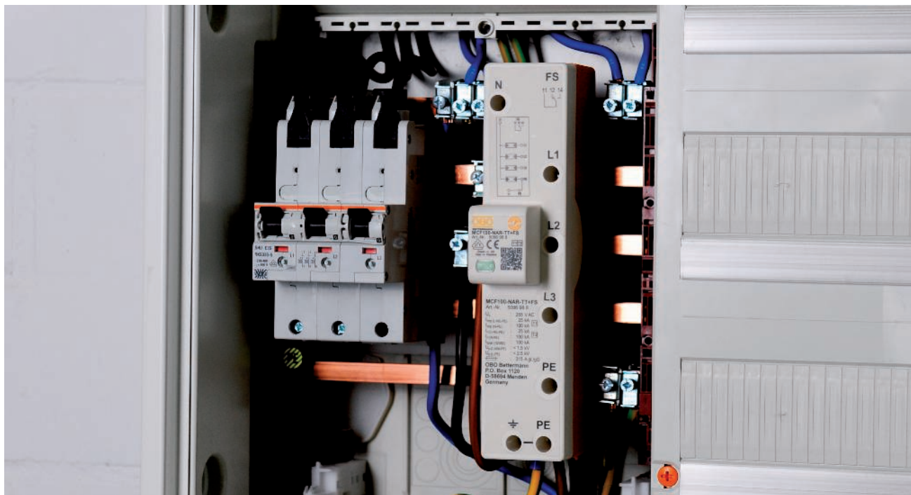
Type 1+2 combination arrestor MCF...NAR on the 40-mm busbar in mains-side connection compartment
