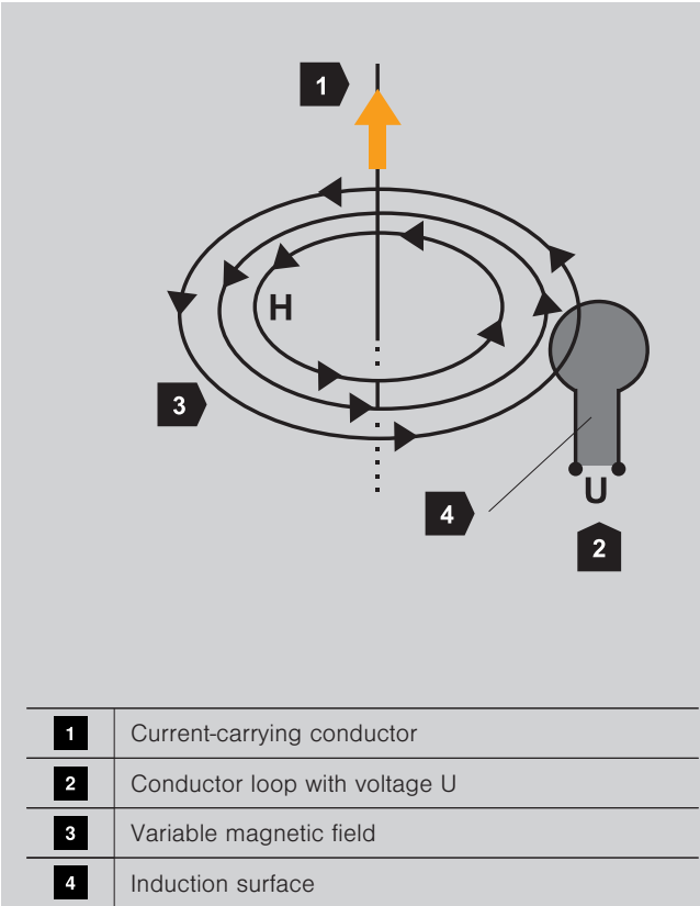
Induction in a conductor loop
