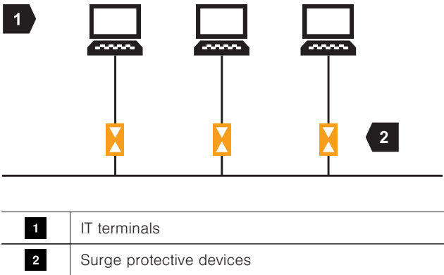
Bus topology
