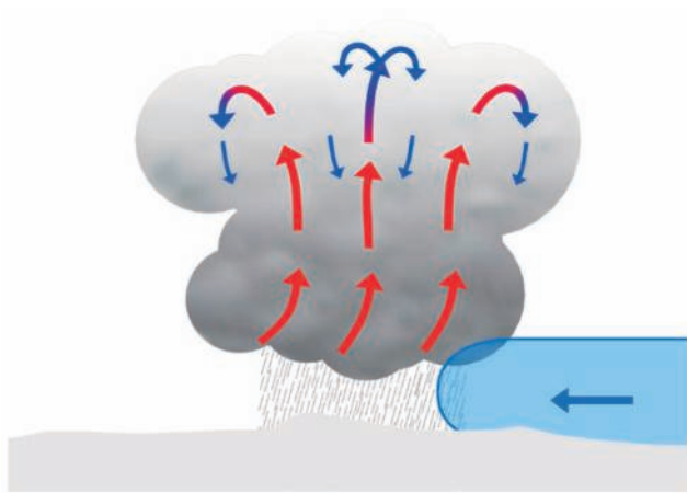
A cold front
