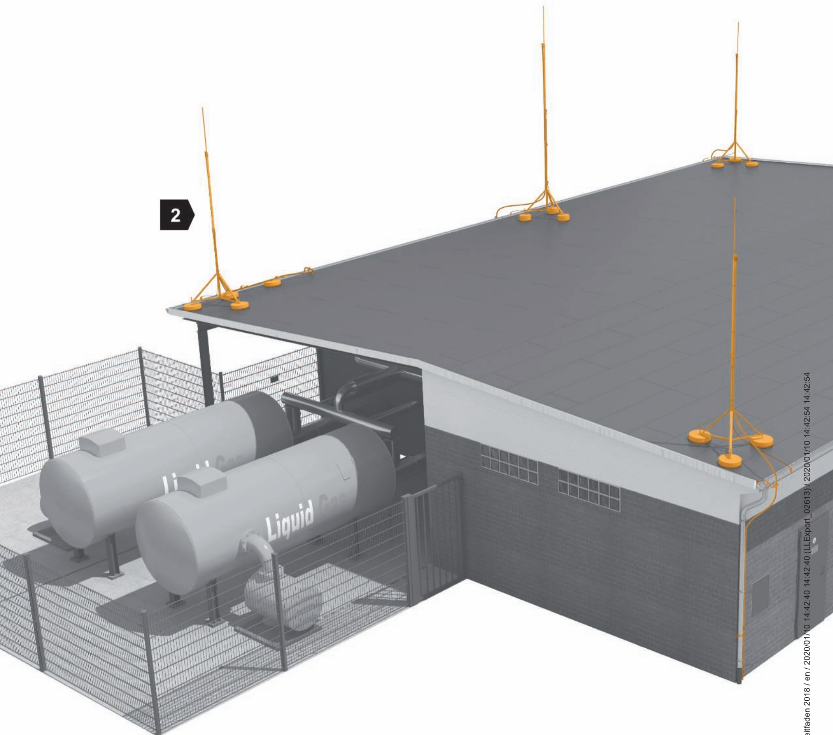
Installation principle for isCon® in potentially explosive areas
