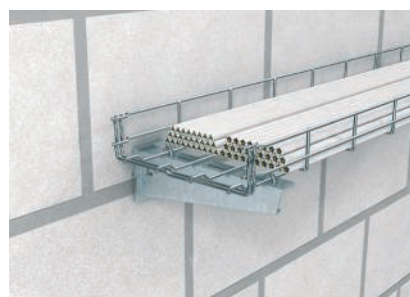
Reference laying type: E, F or G Cable or installation cable on mesh cable trays, e.g. type GR- Magic®
